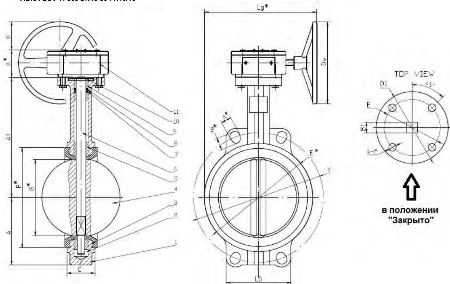
ABRA-BUV-VF863 DN40-80 PN10/16
