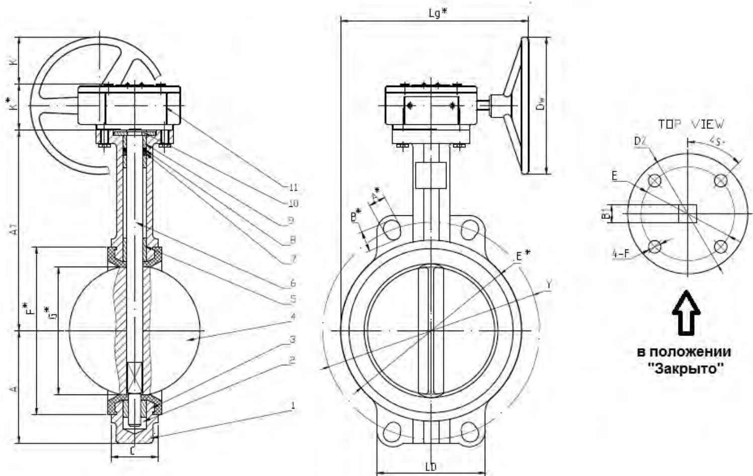
ABRA-BUV-VF866 DN40-80 PN10/16
