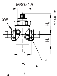
Weld-on tailpieces
